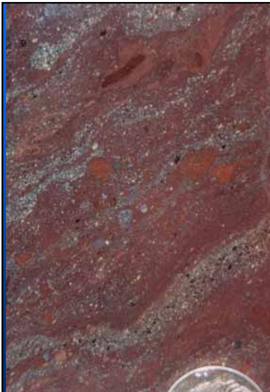
Chalcopyrite-haematite-flourite breccia displaying hydrothermal fluid flow layering
