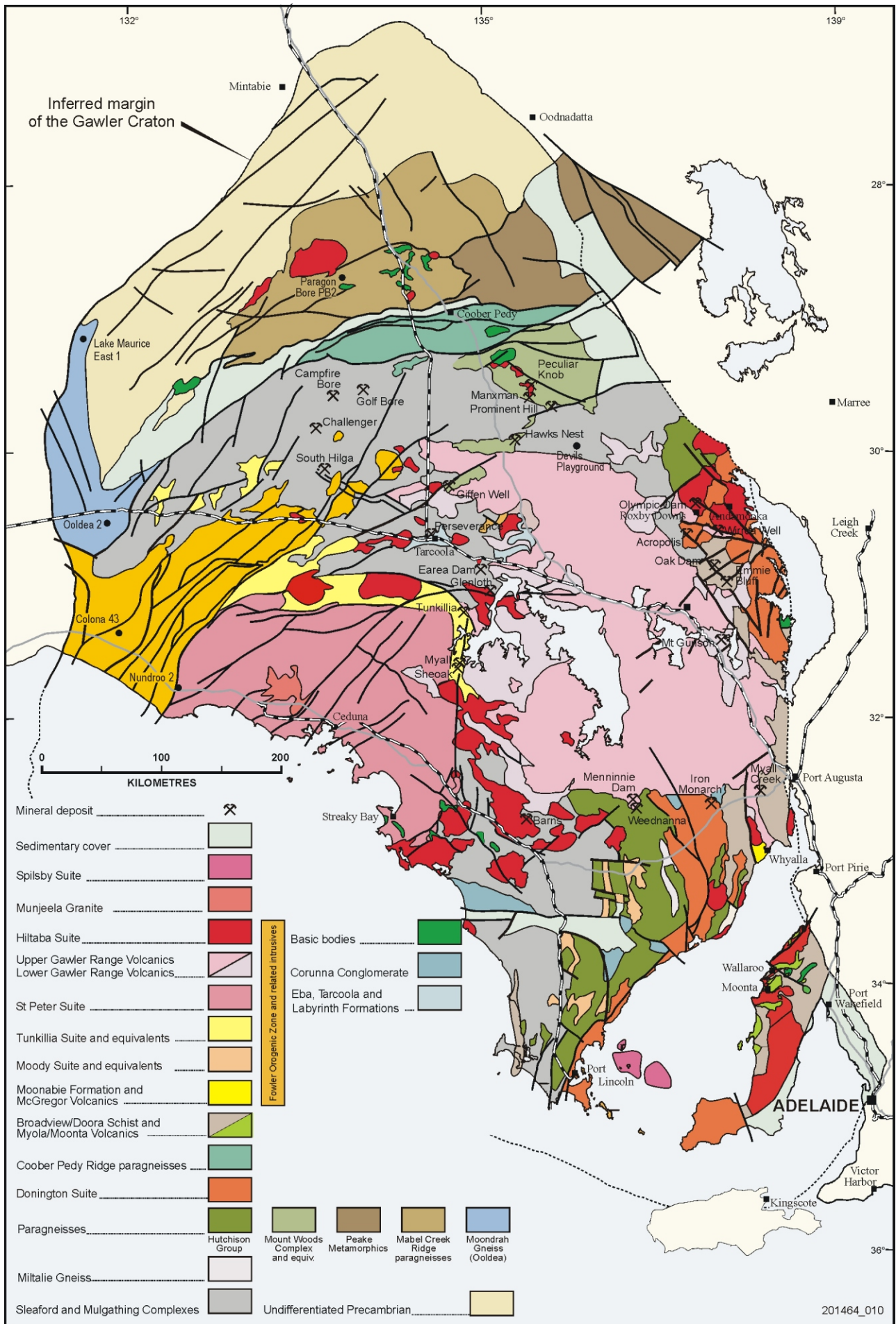
Interpreted subsurface geology of the Gawler Craton, South Australia (Modified after Daly, 1998).
